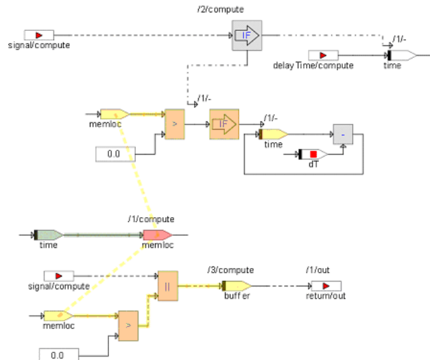
Figure 1: Signal Flow View for ASCET.
