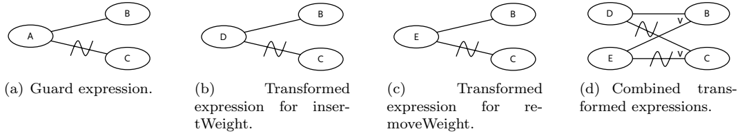
Figure 3: Cause-effect graphs for OCL expressions.
